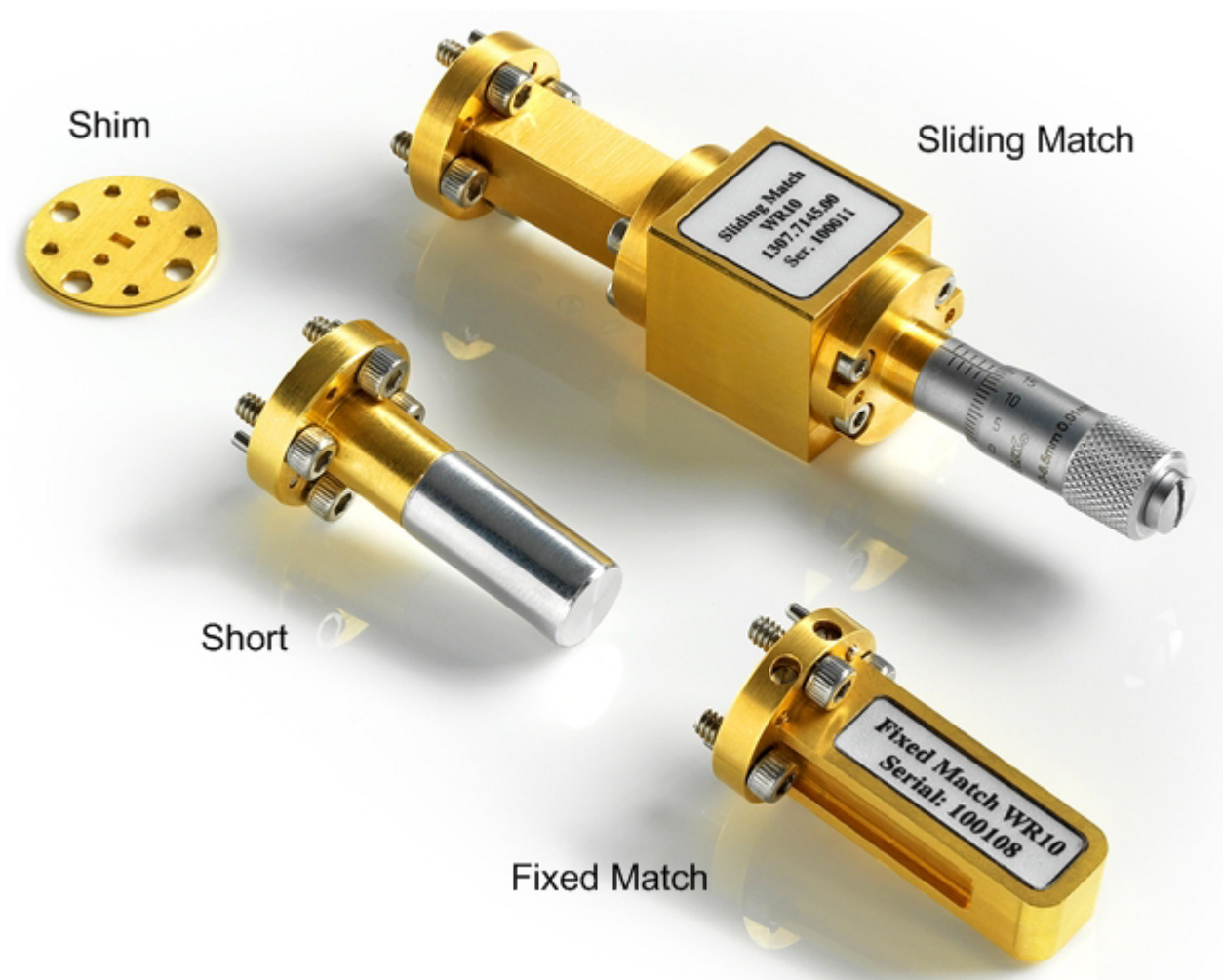
Calibration Kit R&S ZV-WR10 (1307.7100.11)
